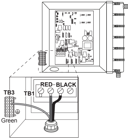
Figure 6 ProTouch™ Control Box Main Terminal Block Connections Diagram
