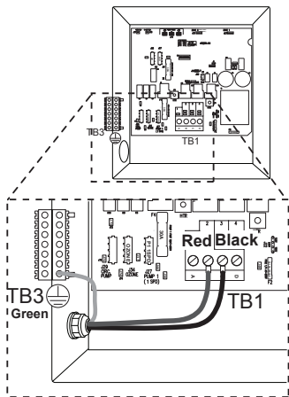
Figure 16 3-Wire, 240 VAC Connection for models (For hard-wired connections only)
