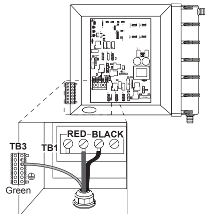
Figure 9 3-Wire, 240 VAC Connection (Hard-wired connections only)
