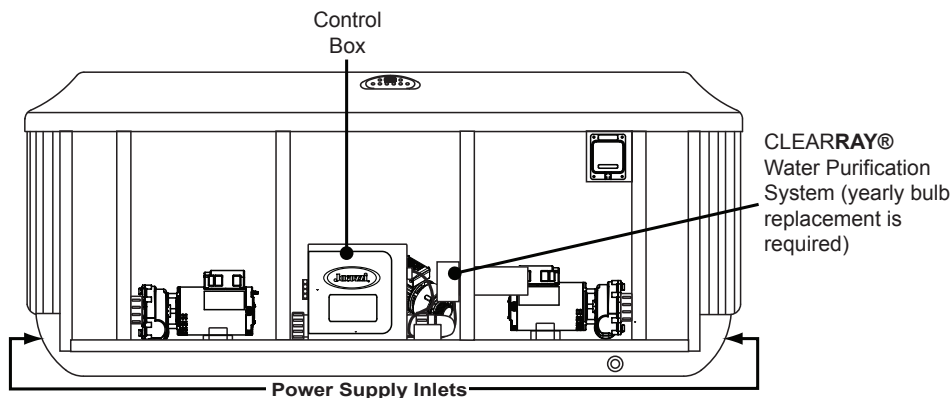
Figure 14 Spa Equipment Compartment (spa features subject to change without notice)
