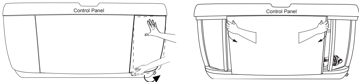
Figure 3 Remove each corner skirt panel followed by the center panels to gain access the spa power terminal block.
